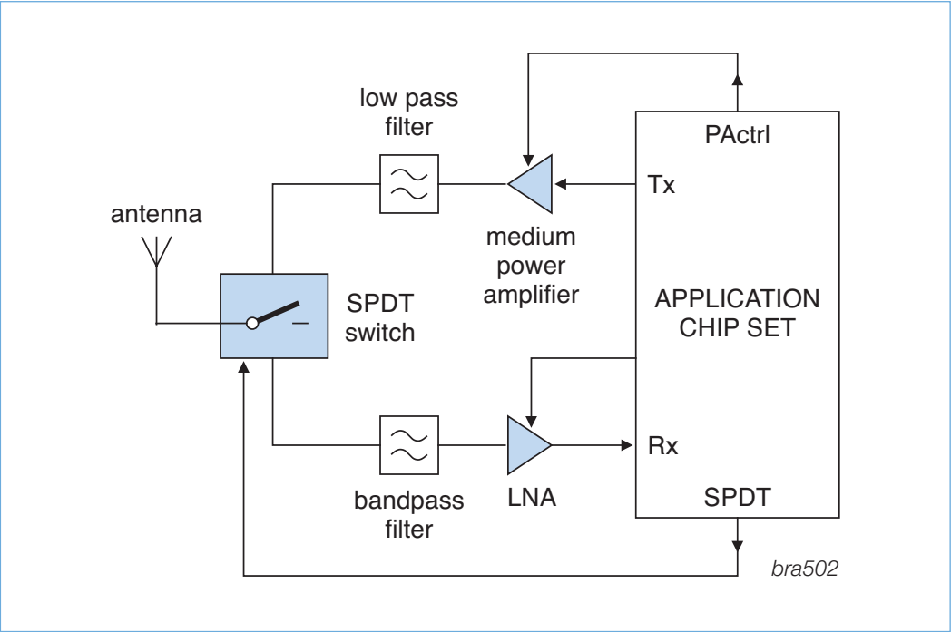
Application diagram
