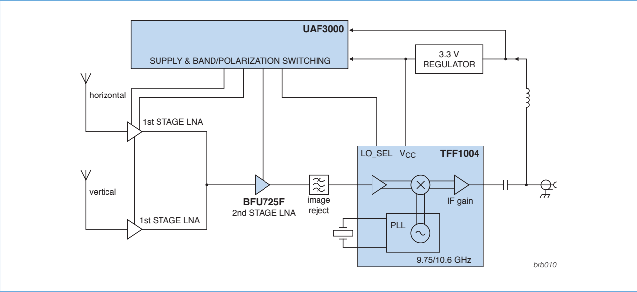
LNB application with TFF1004HN, UAF3000TS, and BFU725F
