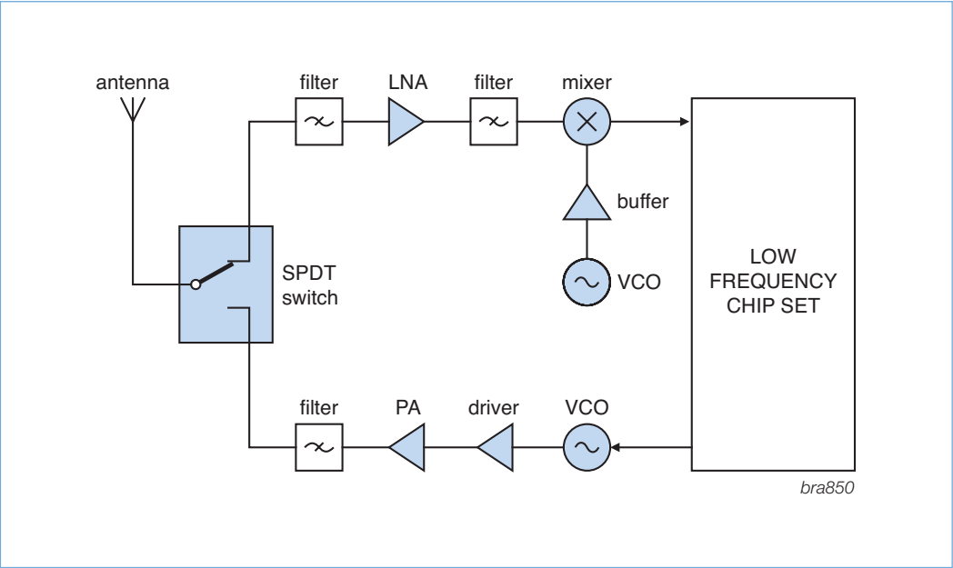
Application diagram
